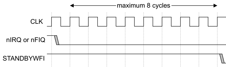
Figure 10-9 STANDBYWFI deassertion
